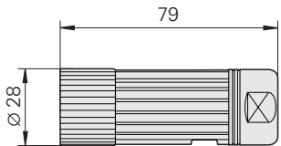
Connector
