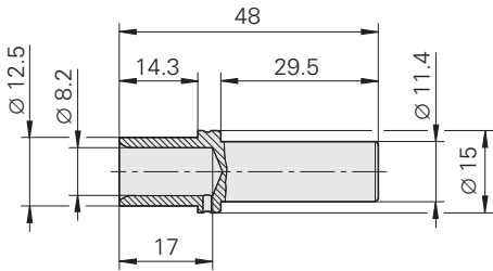
Female contact
